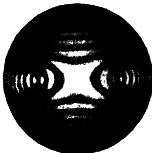
FIG. 58.—Appearance a Minute or so later, the Axes approaching the Centre. Temperature of Crystal about 75^{\circ} C.
